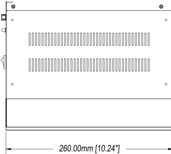
Figure 3-6: RK-8005 Side View
