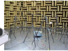
92 mm Fan 3000 RPM, 60 CFM, 38 dBA
