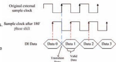
External Clock @ Rising edge Sampling --- 180-degree phase shift
